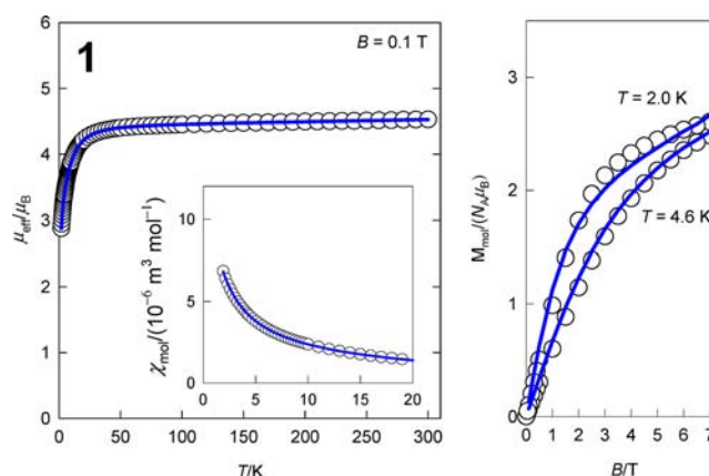
Figure 3. Magnetic data for complex 1 (circles, experimental; lines, simulated, based on best-fit parameters as listed in Table 2). R(\chi) = 0.0038 , R(M) = 0.0312 .
