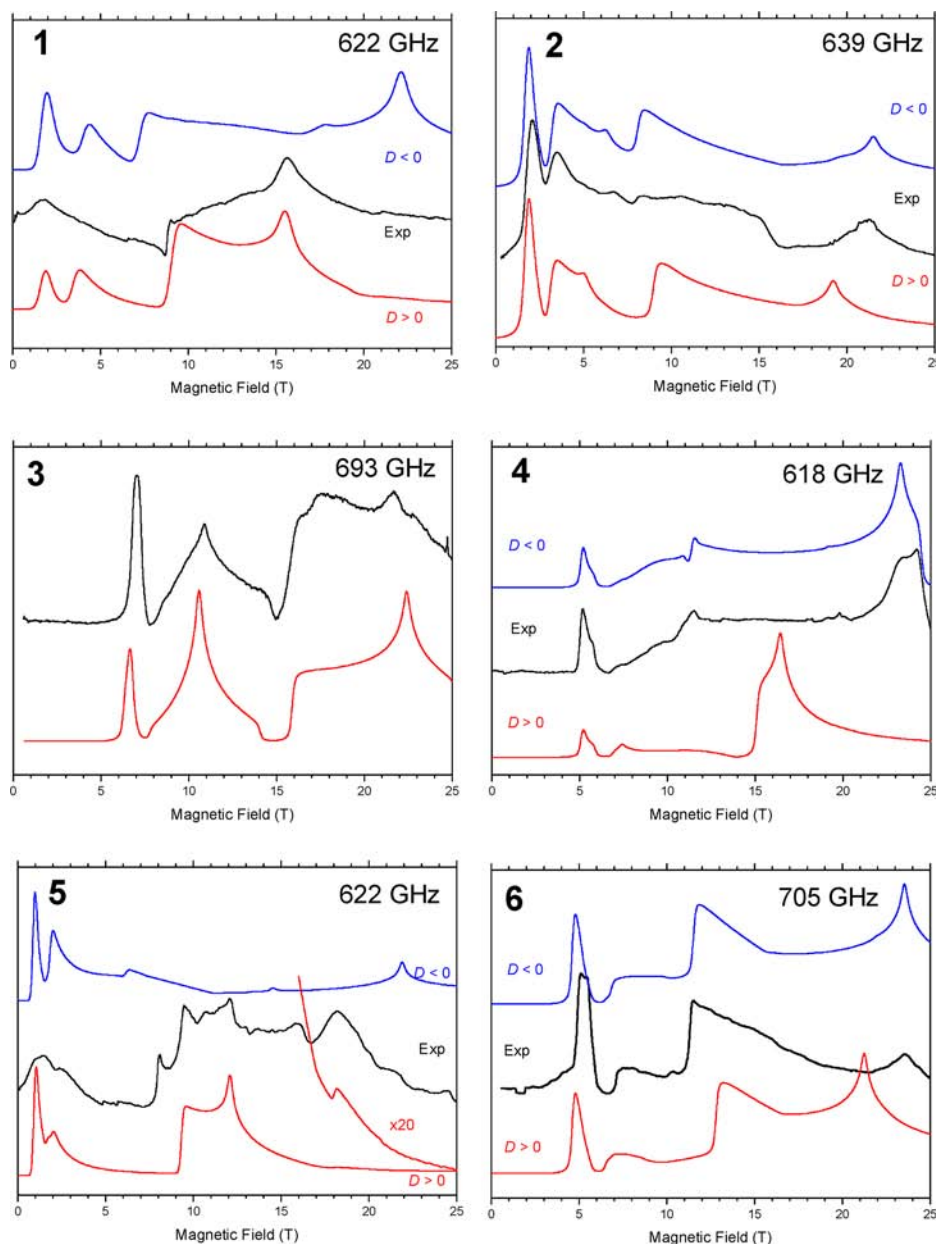
Figure 4. Experimental HFEPR spectra of the complexes studied as pellets at 4.2 K near the top range of frequencies (indicated in each plot) and their simulations assuming a powder distribution of crystallites under the same conditions. The spin Hamiltonian parameters used in the simulations were those obtained from a fit to the 2-D field/frequency map as in Table 2. The submillimeter waves were chopped instead of modulating the magnetic field resulting in absorptive shape. Notes for 3: The small sharp peak near 25 T belongs to a DPPH marker. Simulation parameters are as in Table 2 except for E that was fixed at the maximum rhombicity condition ( E = 1/3 D ). Notes for 5: The spin Hamiltonian parameters used in the simulations were |D| = 9.15 \text{ cm}^{-1} , |E| = 0.93 \text{ cm}^{-1} , and \mathbf{g} = [2.62, 2.62, 2.45] . The red trace magnified by a factor of 20 points out a parallel turning point that is prominent in the experiment, but barely visible in the simulation. This illustrates the nonrandom distribution of the crystallites even in a pellet.
