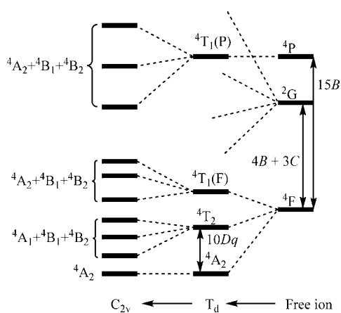
Figure 7. Diagram of crystal-field terms for the pseudotetrahedral Co(II).
