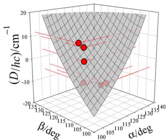
Figure 8. Angular mapping of the zero-field splitting D parameter for pseudotetrahedral \text{Co}(\text{II}) complexes (surface). All crystal-field poles F_4 = 5000 \text{ cm}^{-1} , B = 900 \text{ cm}^{-1} . Circles, experimental data.
