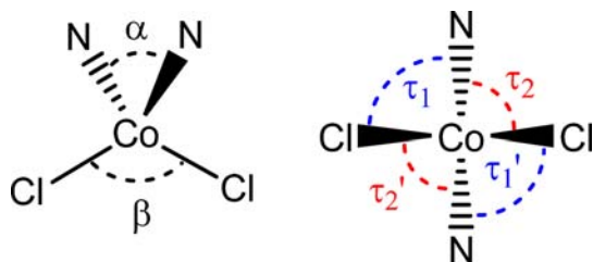
Figure 2. Labeling of bond angles in the \{\text{CoN}_2\text{Cl}_2\} chromophore.
