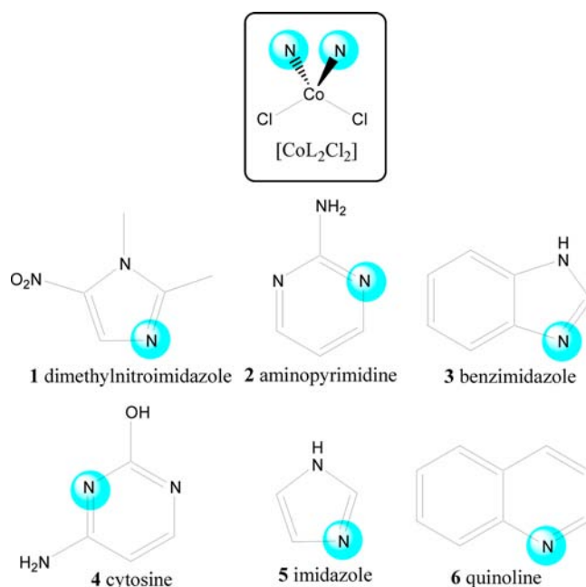
Figure 1. A general molecular structure of the complexes under study and those of the ligands. The donor nitrogen atoms are highlighted.
