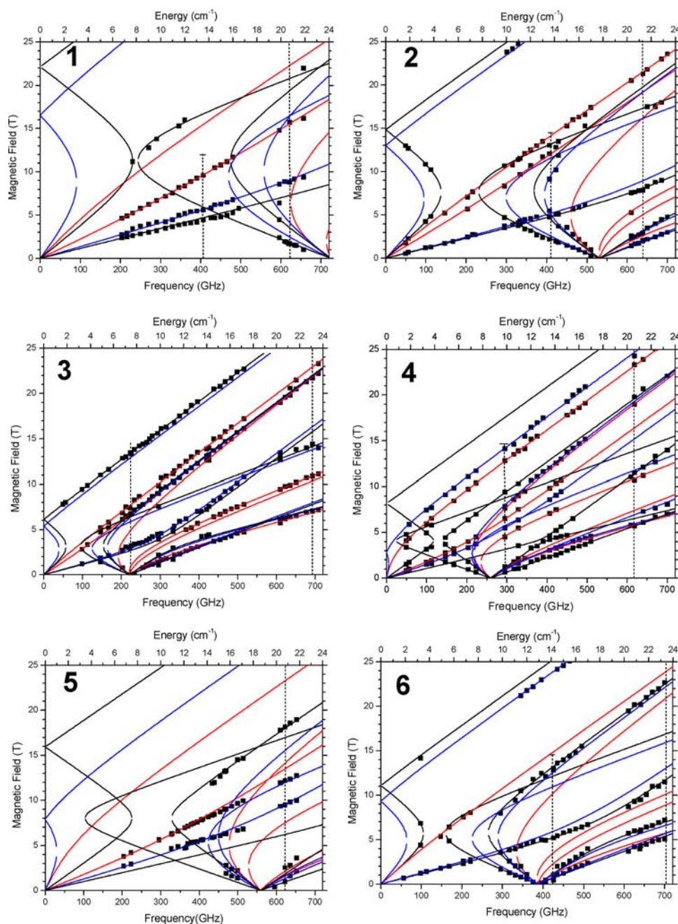
Figure 5. The 2-D maps of turning points in studied complexes as pellets as a function of mm- or submm wave frequency at 4.2–10 K. The squares are experimental points, while the lines were simulated using spin Hamiltonian parameters as in Table 2. Red lines: turning points with B_0//x axis of the ZFS tensor. Blue lines: B_0//y axis. Black lines: B_0//z axis. The dashed lines indicate the frequency and field range of the spectra shown in Figure 4 and Figures S4, S7, S9, S10, and S11, respectively.
