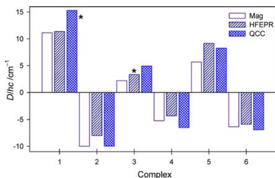
Figure 6. Comparison of the D values obtained by different methods. Asterisk denotes situations when a determination of the sign of the D parameter is impossible; for these cases, the sign has been assigned according to other methods. Abbreviations: Mag, Magnetometry; HFEP, High-Frequency and -Field Electron Paramagnetic Resonance; QCC, Quantum-Chemical Calculation.
